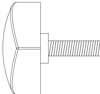
Triangular knob: (M8)
